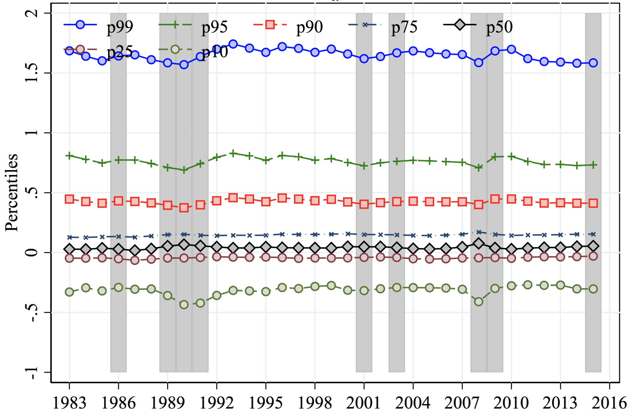
Percentiles of \Delta^1 \varepsilon_{it} for Sample: Men
