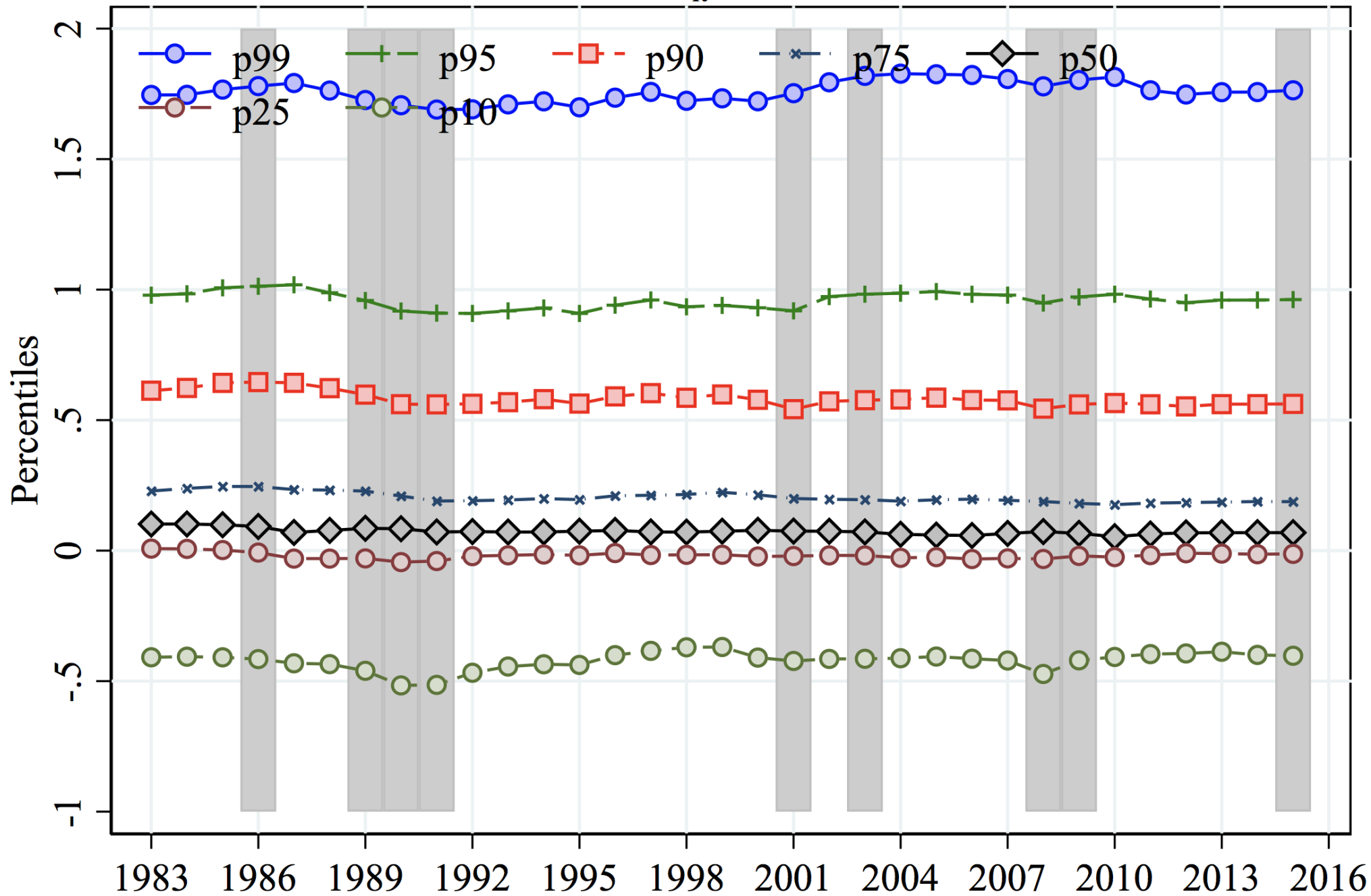
Percentiles of \Delta^1 \varepsilon_{it} for Sample: Women
