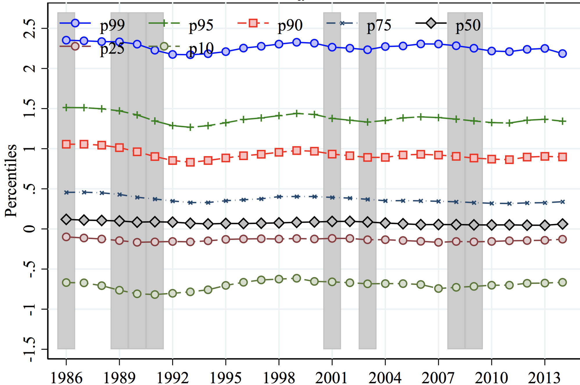
Percentiles of \Delta^5 \varepsilon_{it} for Sample: Women
